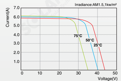
SLP180-24 I-V Curves
