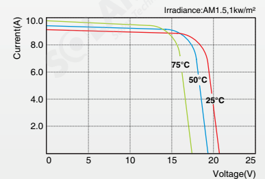
SLP150S-12 I-V Curves
