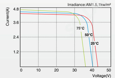
SLP125-24M I-V Curves
