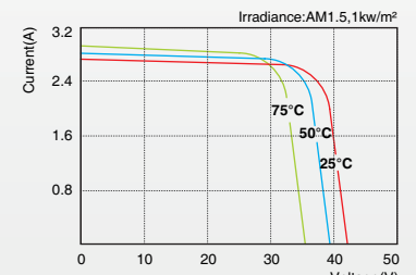
SLP085-24U I-V Curves
