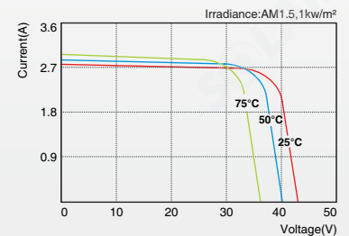
SLP085-24M I-V Curves
