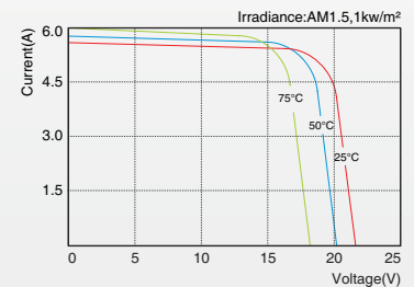
SLP085-12MKCT I-V Curves
