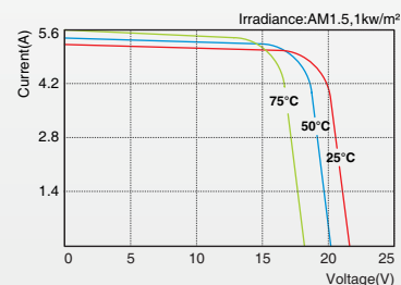
SLP080-12U I-V Curves
