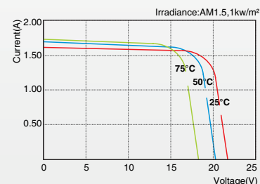
SLP025-12U I-V Curves
