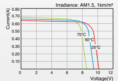
SLP005-06U I-V Curves
